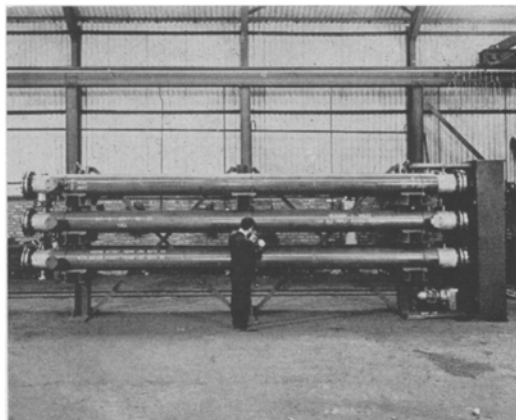
6 shell stearic-oleic crystallizer of stainless steel just delivered for solvent free separation process in U.K. Inner shell size 12 inch.
